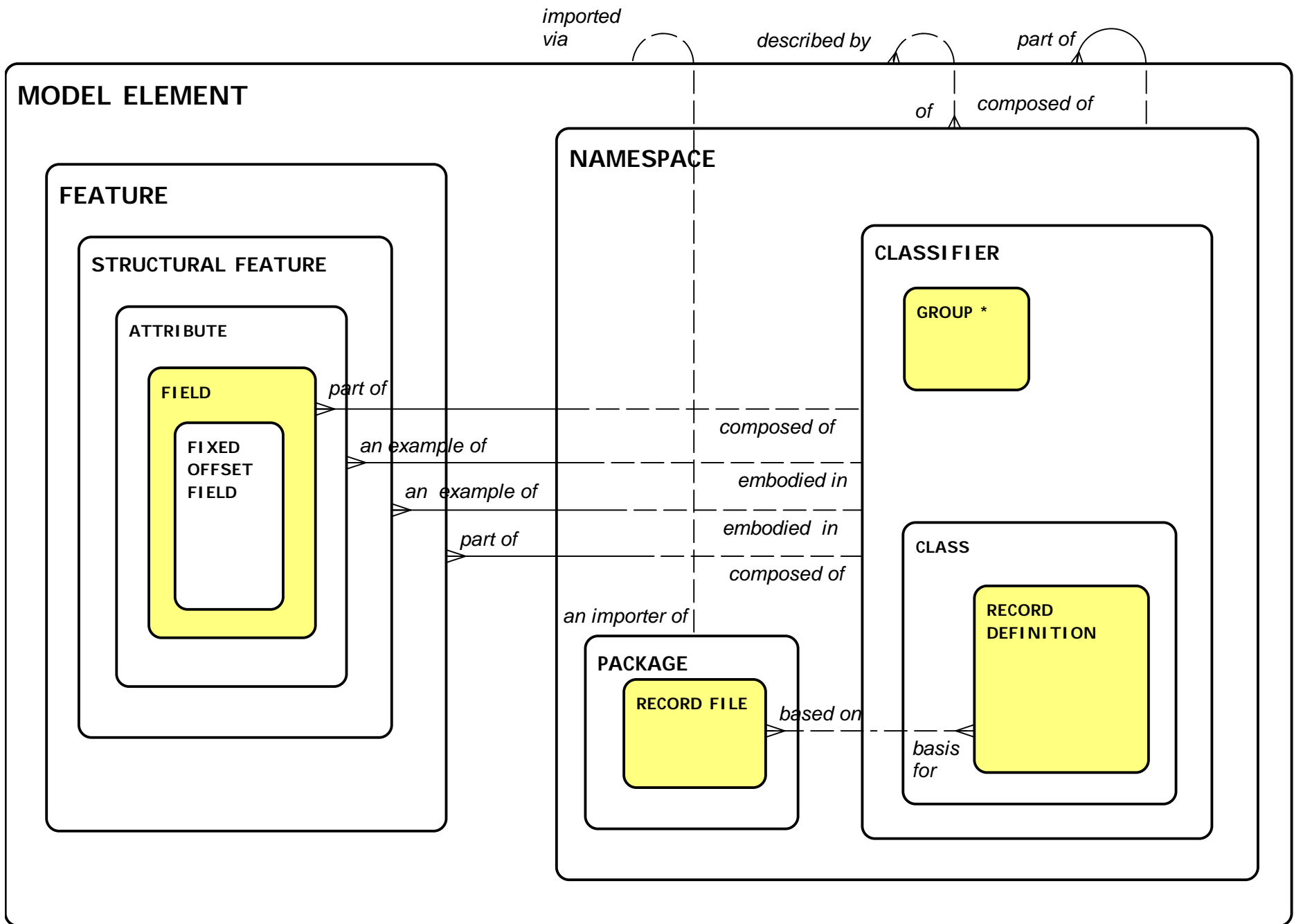
Diagram : FIGURE 4.15 RECORD PACKAG Modified : 15 September 2002 13:56:43 Author : Copyright © 2002 David C. Hay
