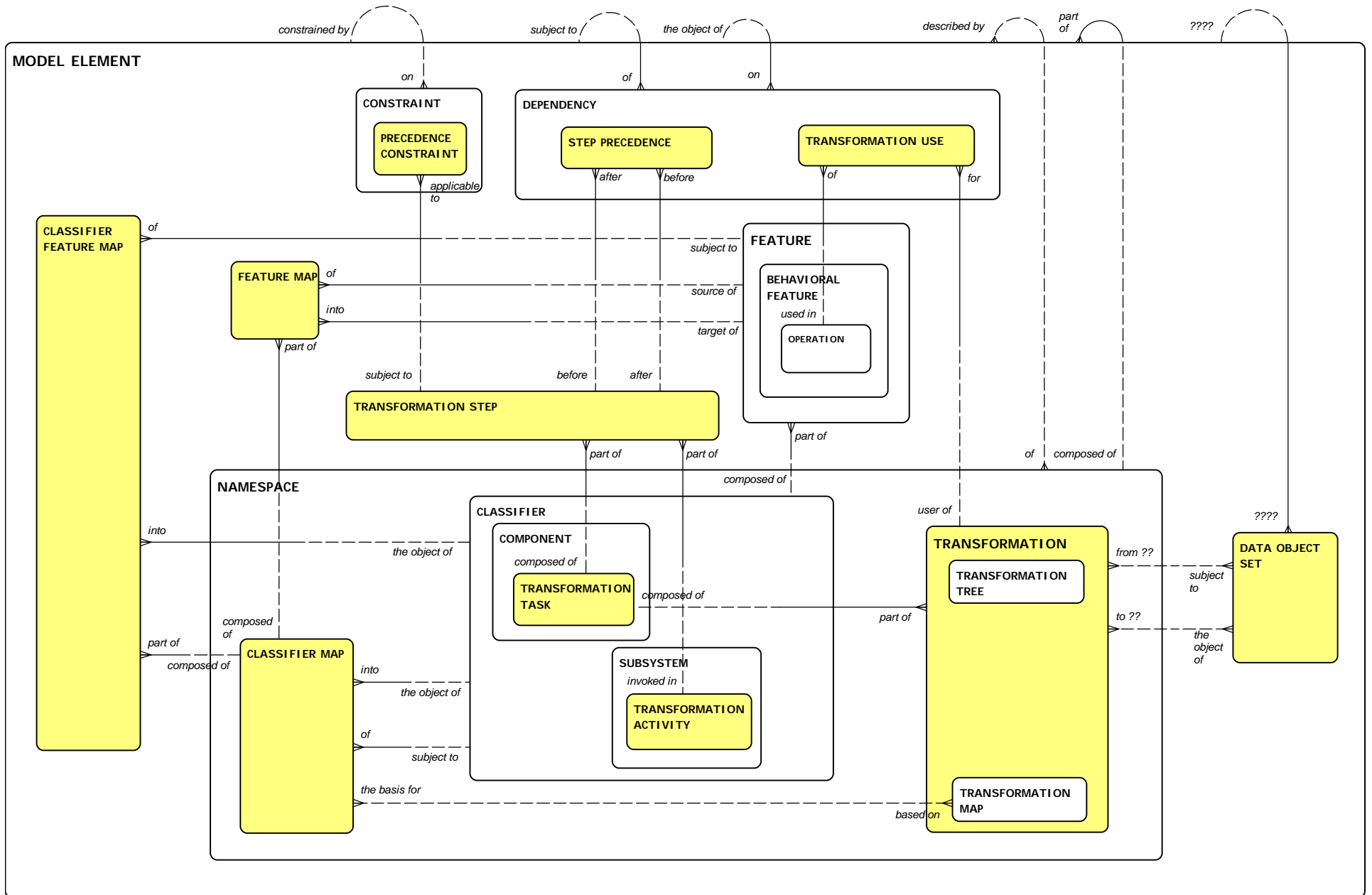
Diagram : FIGURE 4.22 TRANSFORMATION PACKAGE Modified : 15 September 2002 15:24:51 Author : Copyright © 2002 David C.Hay
